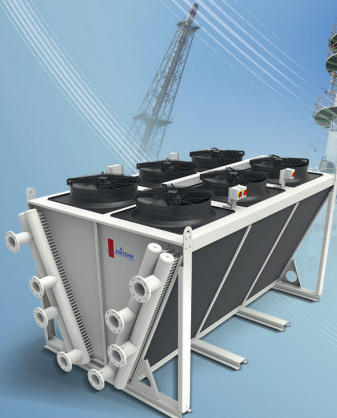
V Type Dry Cooler
